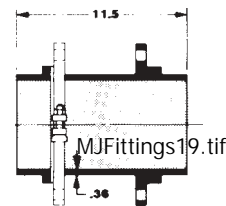
Series 1241 6" x 13" Solid Adapter W/Split Swivel Anchor Gland 31 lbs.
