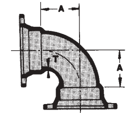
MJ 90° Bend
