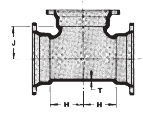
MJ Tee
