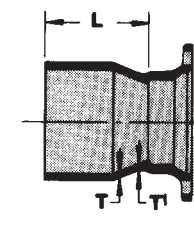
MJ Small End Reducer
