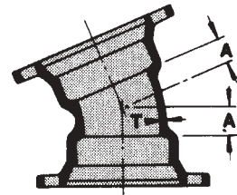
MJ 22 1/2° Bend
