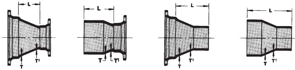
MJ Reducer 1250- MJ Small End Reducer SEB 1251- MJ Large End Reducer LEB 1252- PE x PE Reducer 1257-
