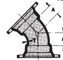
MJ 45° Bend
