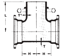
Hydrant Tee
