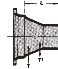
MJ Large End Reducer
