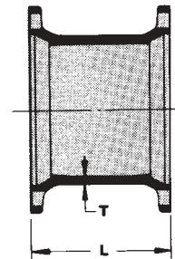
MJ Short Sleeve
