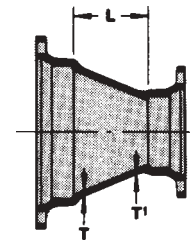
MJ Reducer
