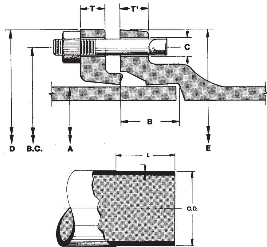
Plain End
